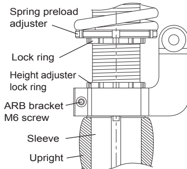
Fig 5 With PDCC
