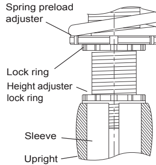
Fig 4 Without PDCC
